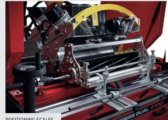
POSITIONING SCALES
